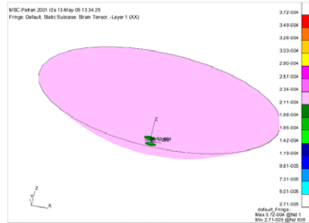
Fig. 5 The strain distribution in longitudinal direction on the upper surface of parabolic antenna reflector by thermal expansion induced from temperature increase from 25°C to 120°C.
