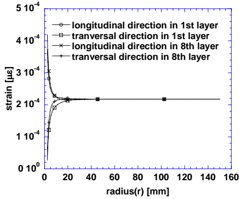
Fig. 6 The strain distribution in longitudinal and transverse direction on the upper(1 st ) and bottom(8 th ) surfaces of parabolic antenna reflector along the radius, r .
