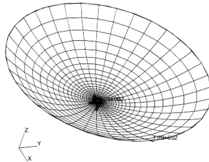
Fig. 3 The FE model for the thermal deformation analyses of the parabolic antenna reflector.
