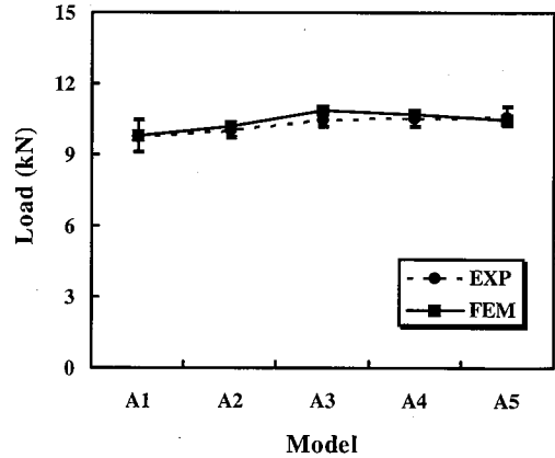
(a) Failure loads with various w/d ratios
