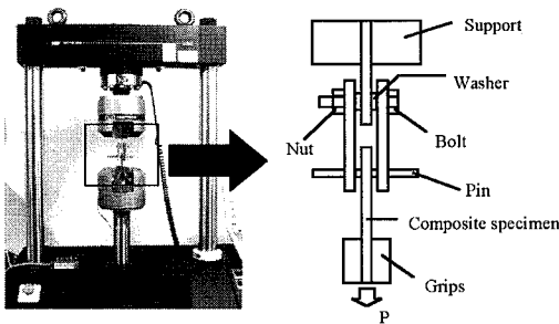
Fig. 11 Experimental set-up.
