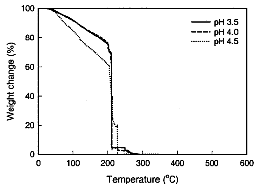
Fig. 8 TGA results of microcapsule constituents under heating up to 600°C (continuous heating).
