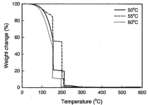
Fig. 11 TGA results of microcapsule constituents under heating up to 600°C (isothermal of 150°C for 2 hours).
