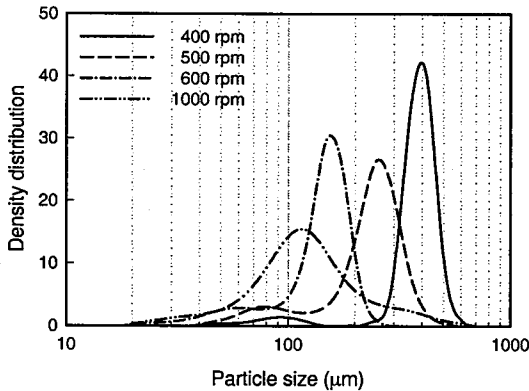
Fig. 4 Particle size distribution of microcapsules.
