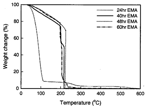
Fig. 6 TGA results of microcapsule constituents under heating up to 600°C (continuous heating).
