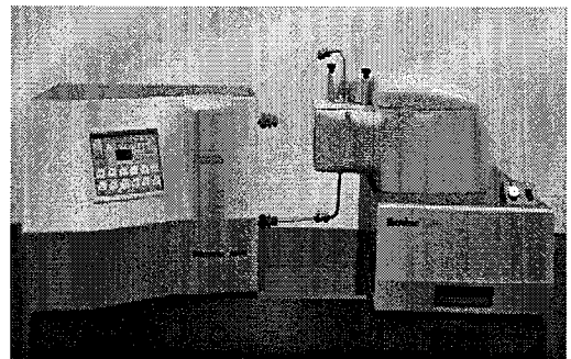
Fig. 2 Particle size analyzer on laser diffraction technique.
