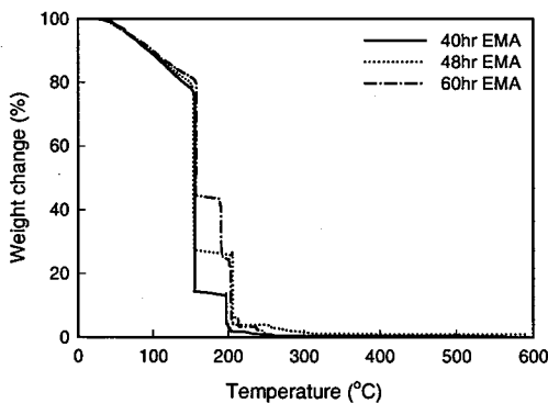
Fig. 7 TGA results of microcapsule constituents under heating up to 600°C (isothermal of 150°C for 2 hours).
