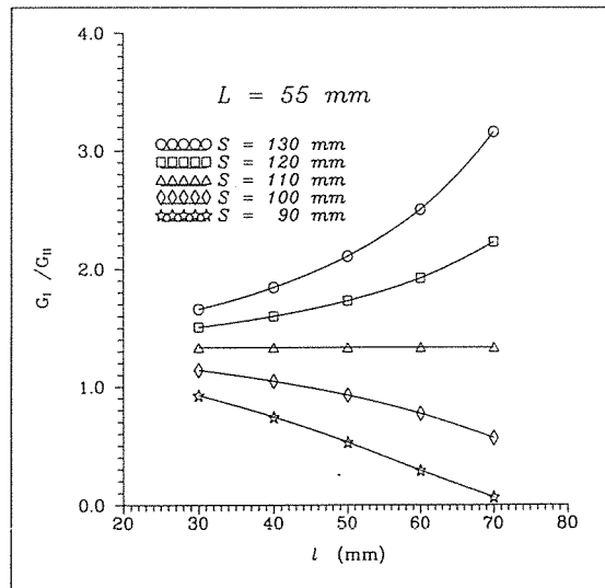
Fig.4. G_I/G_{II} variation for l of modified mixed mode bending specimen
