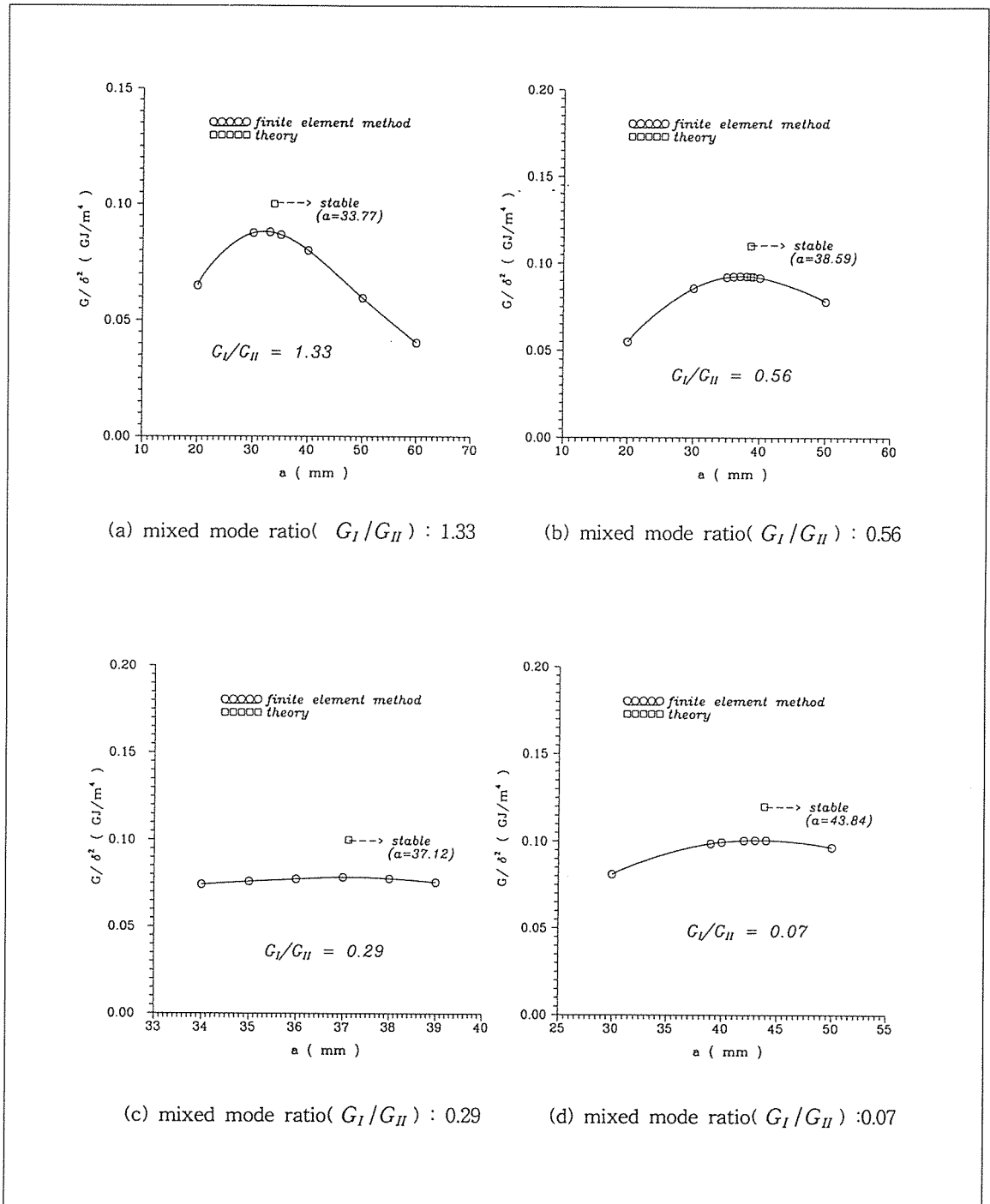
Fig.5. G/\delta^2 variation for crack length of modified mixed mode bending specimen
