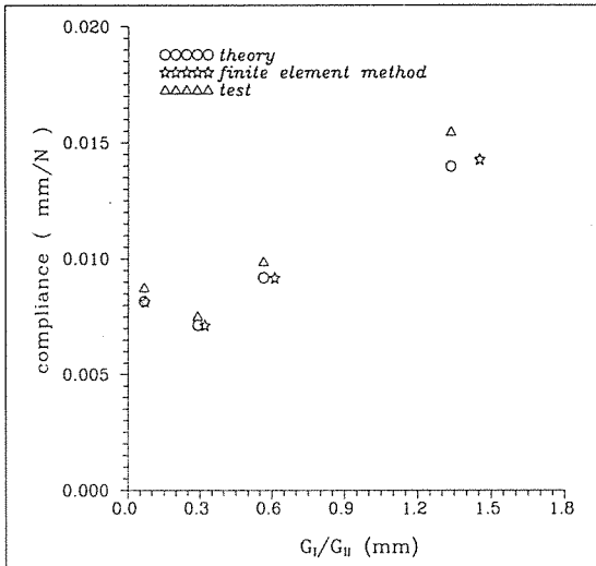
Fig.6. Compliance for G/G_{II} of modified mixed mode bending specimen
