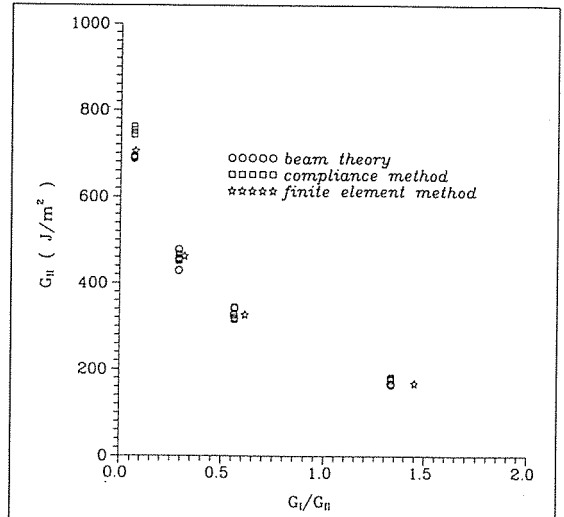
Fig. 9. G_{II} variation for G_I/G_{II} ratio of modified mixed mode bending specimen
